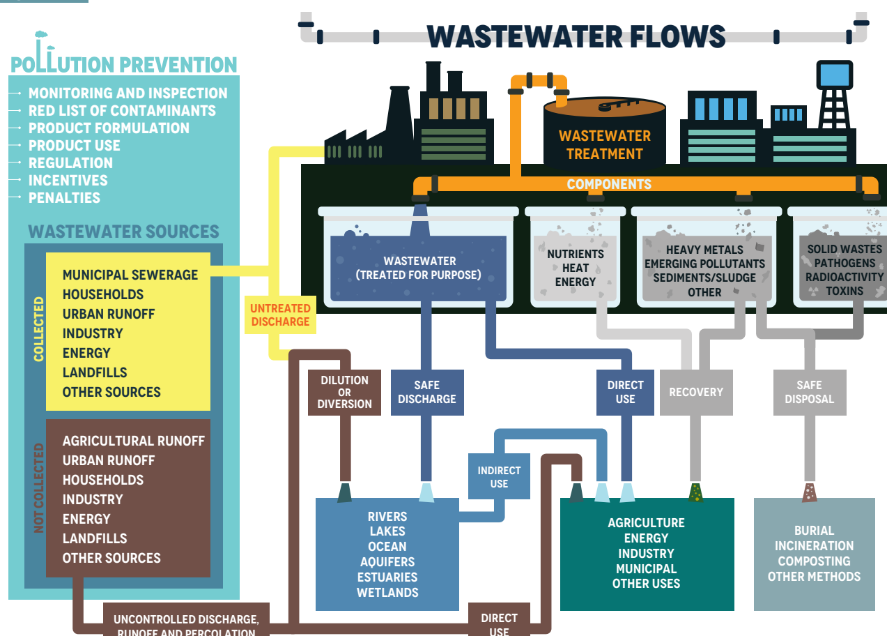
Figure 1.2 Wastewater flows
