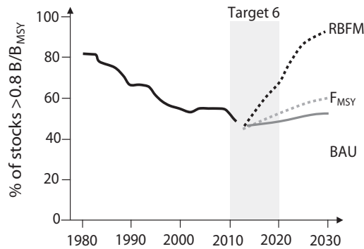
Figure 12. Projected trajectories of the global proportion of sustainably fished stocks ( B > 0.8B_{MSY} ) according to different policy scenarios. RBFM = Economic optimization policy. F_{MSY} = Biological optimization policy. BAU = business-as-usual with presently well-maintained fisheries maintained as such, and other fisheries declining under poor or no management. Modified and redrawn from Costello et al., (2016). The Target 6 decade is indicated to signal that large uncertainties still exist about the likely situation in 2020.
