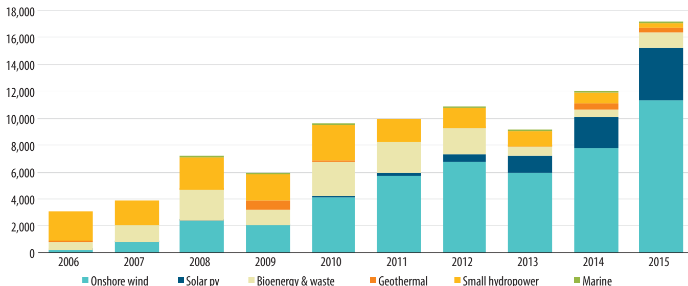
FIGURE 26: Investments in renewables are rising rapidly in Latin America, driven by onshore wind
