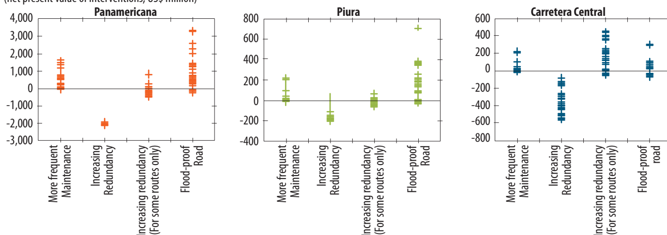
FIGURE 33: Flood-proofing critical road segments in Peru pays off in almost all possible scenarios
