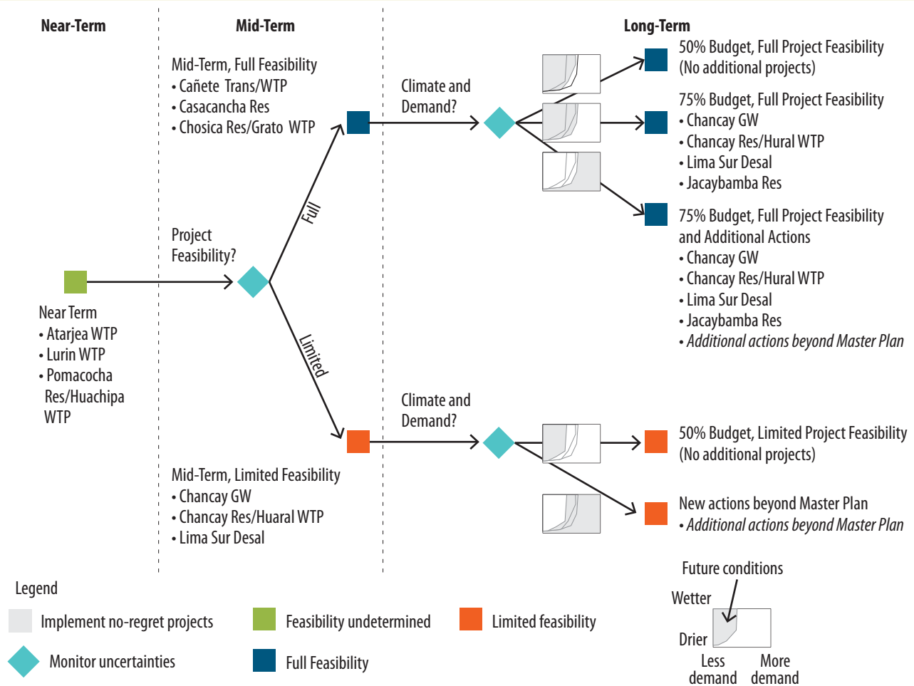
BOX FIGURE 1: Robust and adaptive portfolio of water reservoirs to implement Lima’s Water Resource Master Plan
